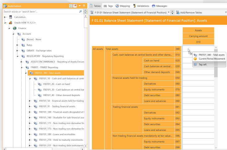
A data point in a template in the FINREP taxonomy being automated via drag-and-drop
